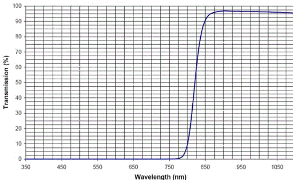
80115 INFRARED LONGPASS (Visible Blocking) FILTER
